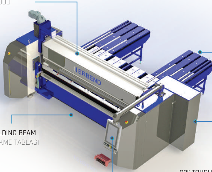
22" TOUCHSCREEN CONTROLLER 22" DOKUNMATİK EKRAN
